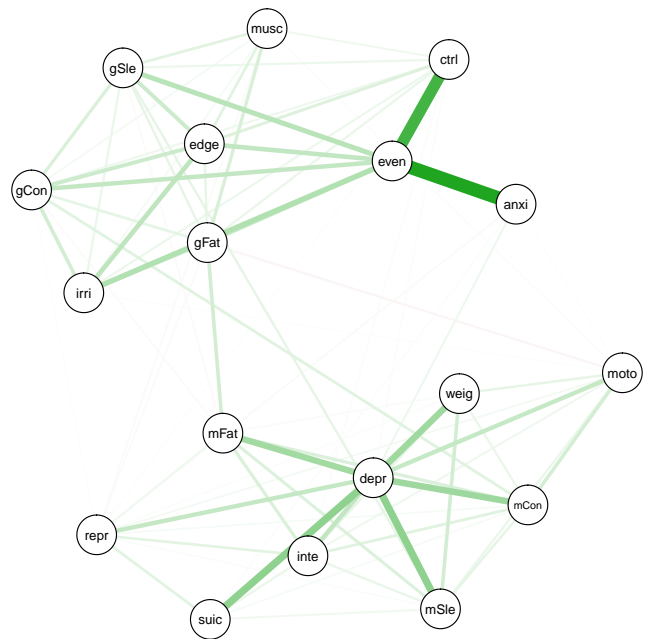
NCS-R --- Ising model
