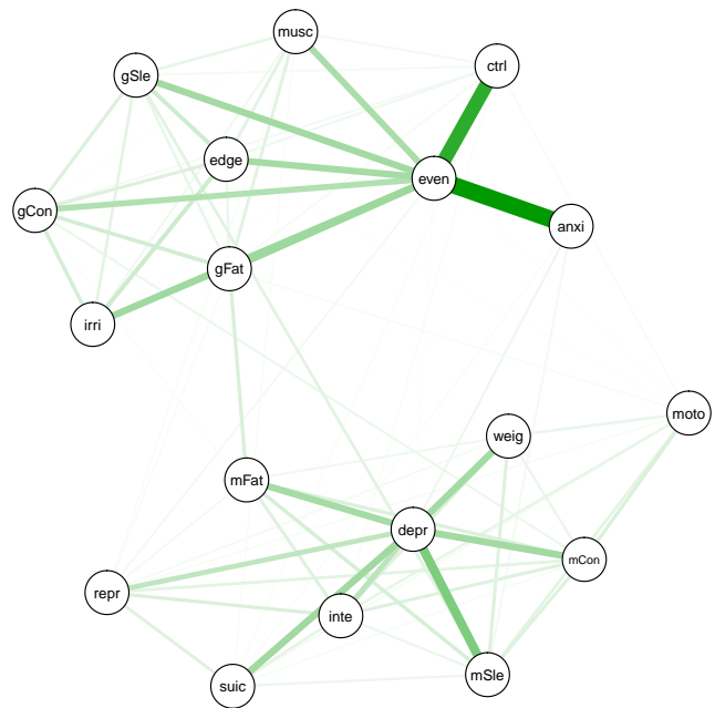
NSMHWB --- Ising model
