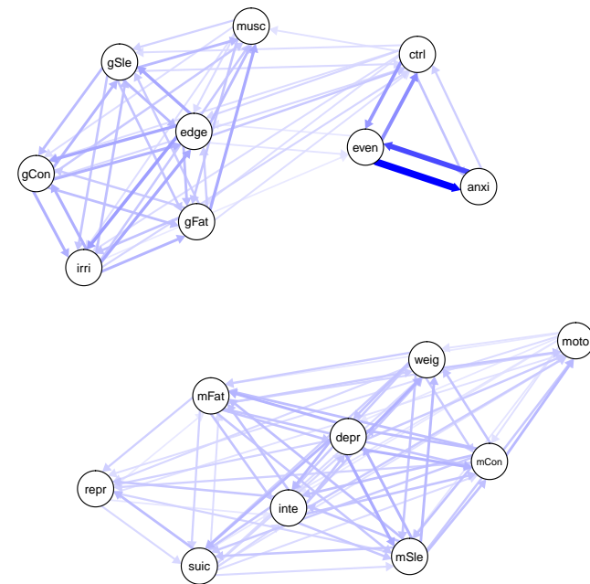
NCS-R --- Censored relative importance
