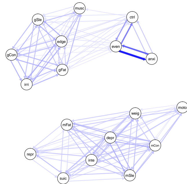
NSMHWB --- Censored relative importance
